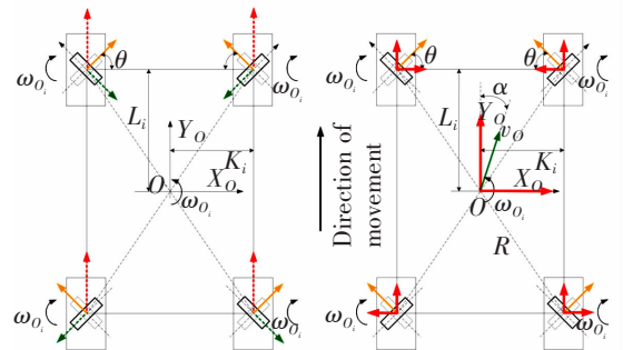
(a) Velocity analysis diagram (b) Establish coordinate system
