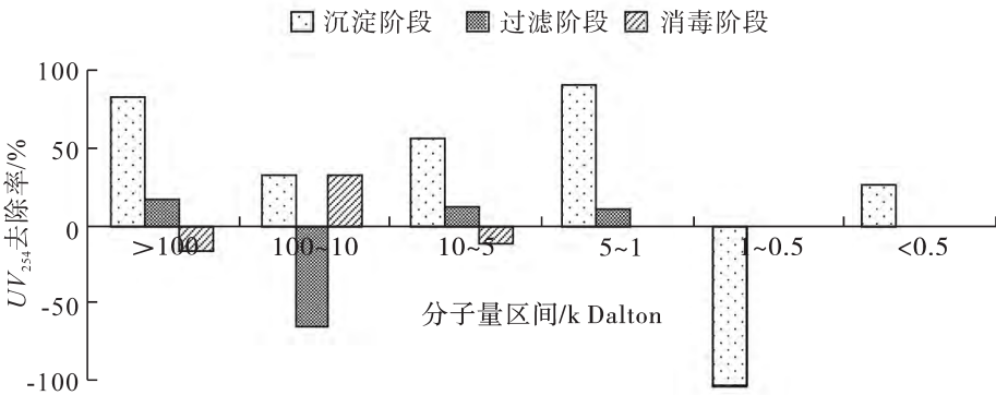
图6 各分子量区间UV 254 去除率 Fig. 6 UV 254 removal rate at different MW ranges
