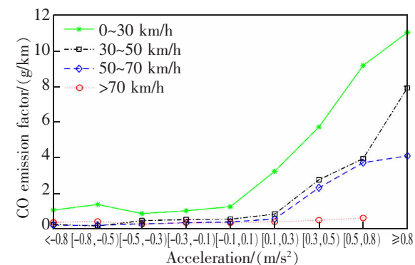
(a) Emission factor of CO
