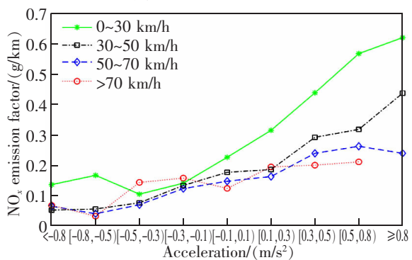
(c) Emission factor of NO x
