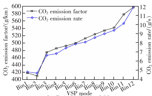
(b) Emission factor of CO 2
