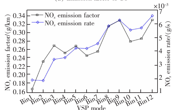
(c) Emission factor of NO x
