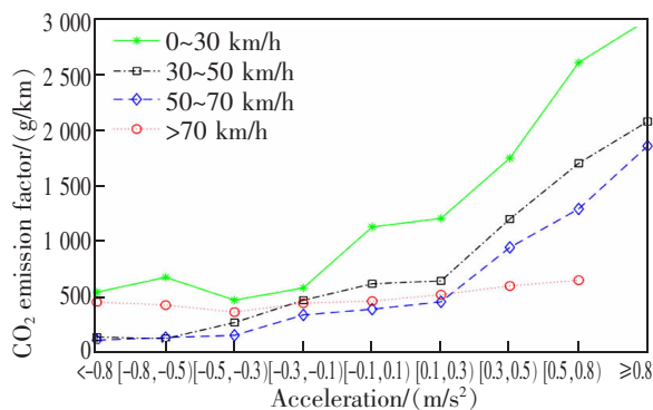
(b) Emission factor of CO 2
