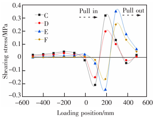
图 12 不同荷载作用位置下过渡区剪应力分布图 Fig.12 Distribution diagram of shearing stress in transition pavement under different load positions
