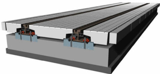
(b) Tram track 3D model
