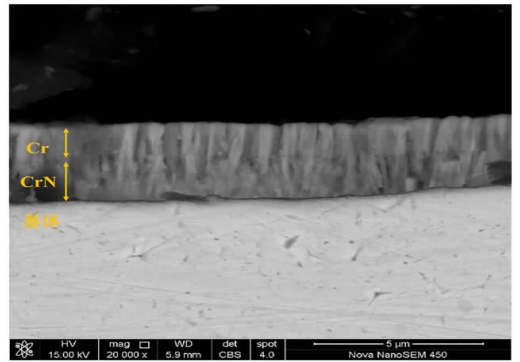
图 3 溅射 Cr 层后涂层断口形貌 Fig.3 SEM of fracture morphology of Cr coating after sputtering
