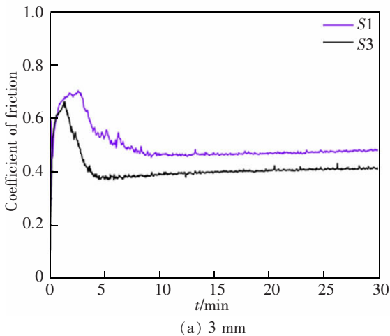
图 4 300 r/min 时 10 N 载荷下不同半径摩擦系数 Fig.4 Coefficient of friction of different radius under 10 N load at 300 r/min
