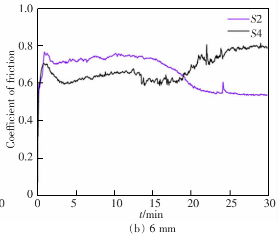
图 4 300 r/min 时 10 N 载荷下不同半径摩擦系数 Fig.4 Coefficient of friction of different radius under 10 N load at 300 r/min
