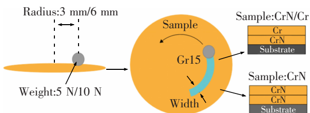
图 1 测试样品与摩擦磨损实验示意图 Fig.1 Test sample and experimental diagram of friction and wear
