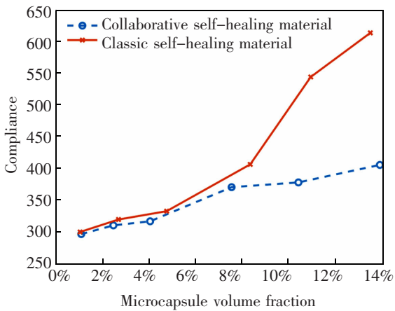
图7 两类自修复材料微胶囊体积分数与柔度关系 Fig.7 Relationship between microcapsule volume fraction and compliance of two kinds of self-healing materials
