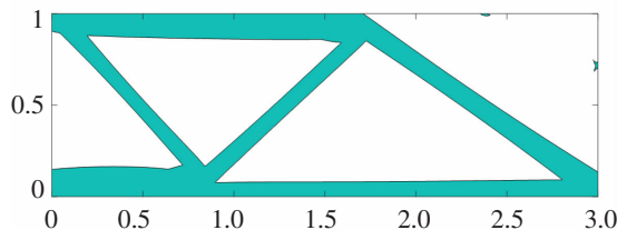
图 6 无胶囊载体拓扑优化构型 Fig.6 Carrier topology optimization configuration (without capsule)
