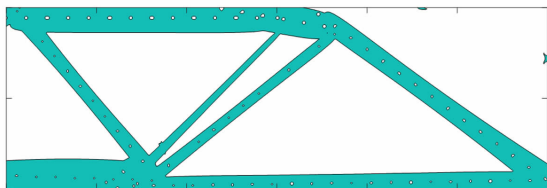
图 5 协同优化自修复材料拓扑优化构型 ( a=0.1, G=0.1 ) Fig.5 Optimize topology and configuration of collaborative self-healing materials ( a=0.1, G=0.1 )
