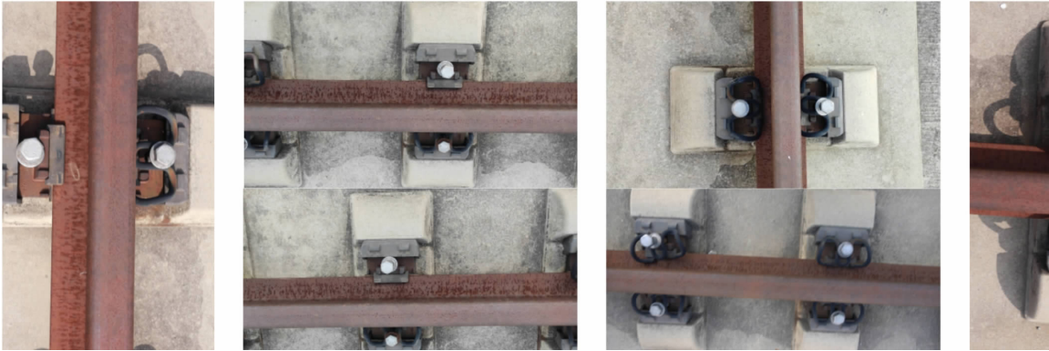
图 5 高铁扣件数据集 Fig.5 High-speed railway fasteners data set
