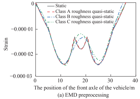
Fig. 8 Mid-span strain of the second span
