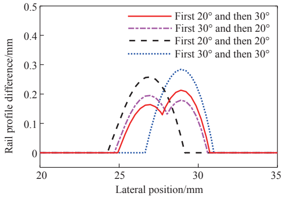
图3 两个砂轮(不同角度)切削后的打磨量曲线 Fig. 3 Curve of grinding amount after cutting with two grinding wheels (different angles)
