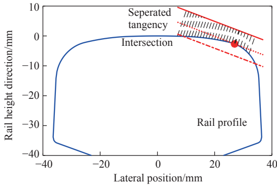
图1 单个砂轮钢轨打磨过程示意图 Fig. 1 The rail grinding process of a single wheel
