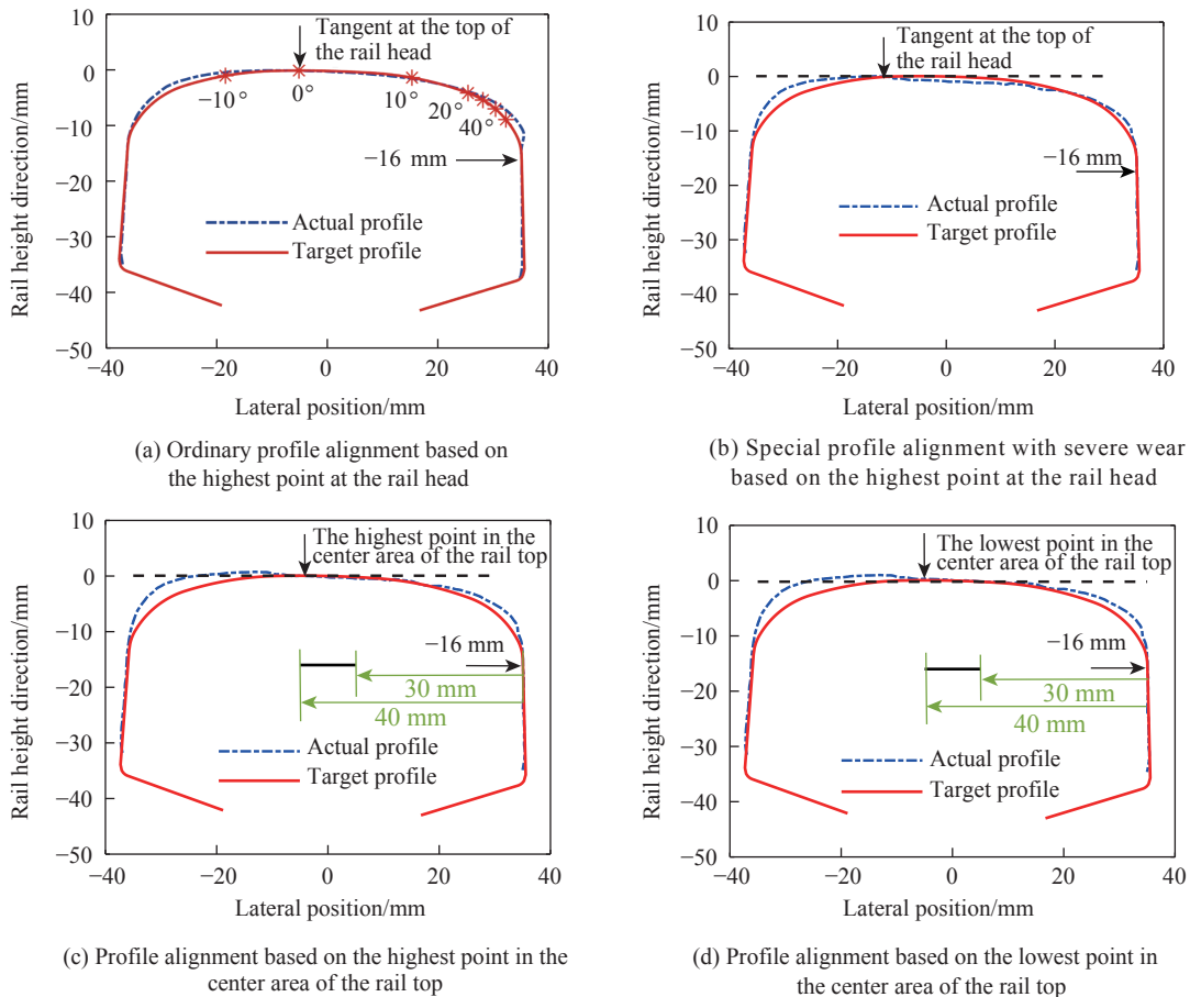
图5 钢轨廓形对齐方式比较 Fig. 5 Comparison of rail profile alignment
