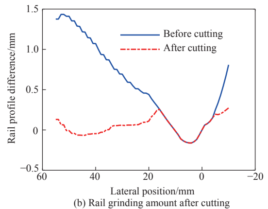
图8 切削完成后的钢轨廓形及钢轨打磨量曲线 Fig. 8 Rail profile and rail grinding amount after cutting
