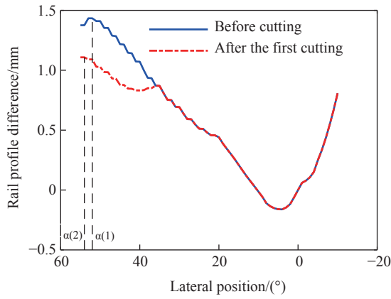
图7 第一遍切削后的钢轨廓形及钢轨打磨量曲线 Fig. 7 Rail profile and grinding amount after the first cutting
