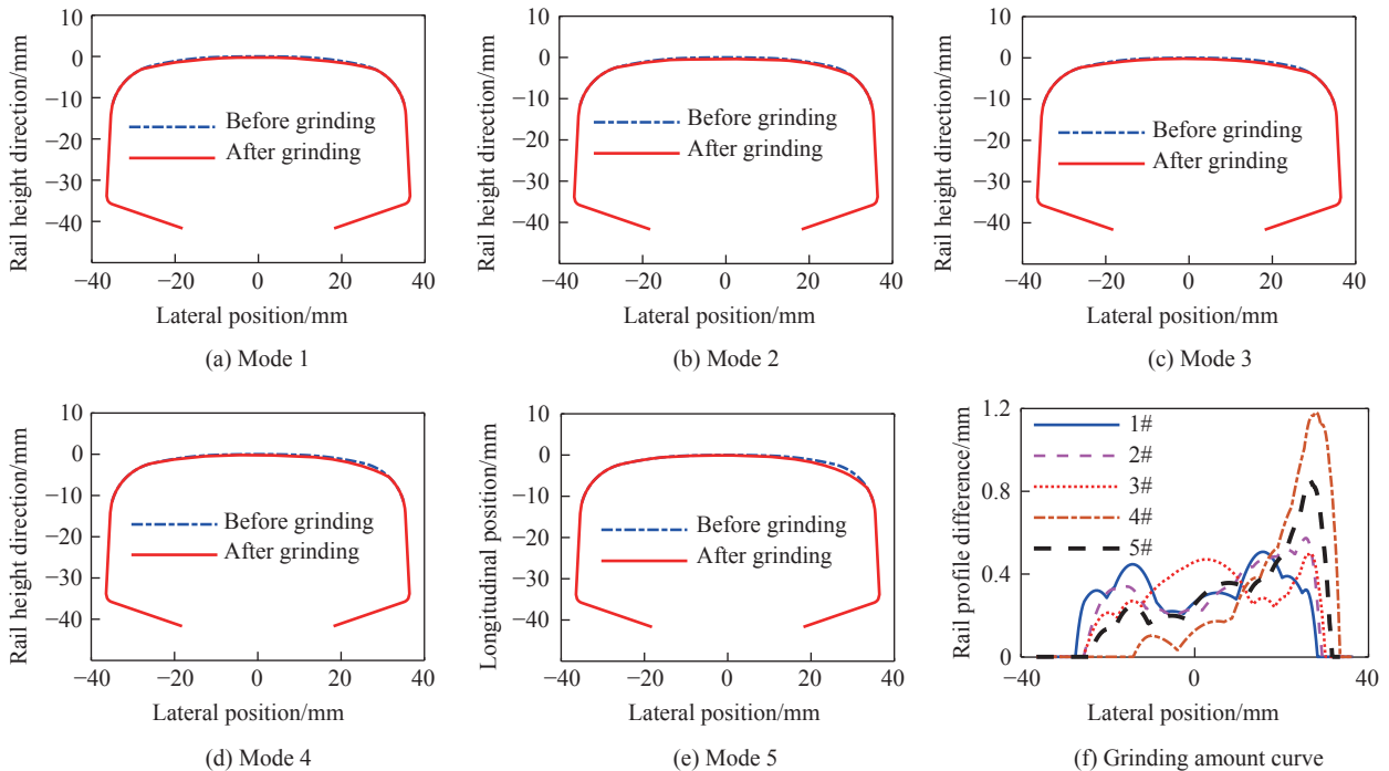
图4 钢轨打磨车常用打磨模式下的切削前后钢轨廓形及打磨量曲线 Fig. 4 Rail profile and grinding amount curve before and after cutting under common cutting mode of rail grinding train
