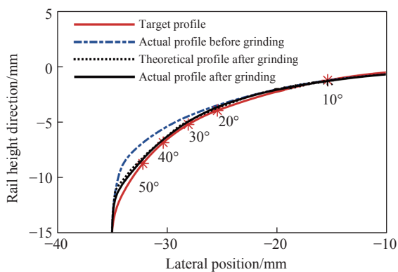
图9 打磨后的钢轨廓形及钢轨打磨量曲线 Fig. 9 Comparison of rail profile before and after grinding
