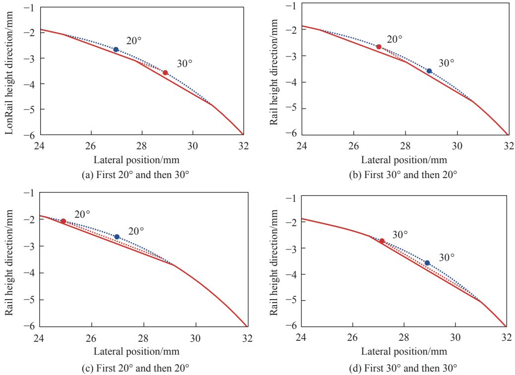
图2 两个砂轮(不同角度)切削后的钢轨廓形 Fig. 2 Rail profile after cutting with two grinding wheels (different angles)
