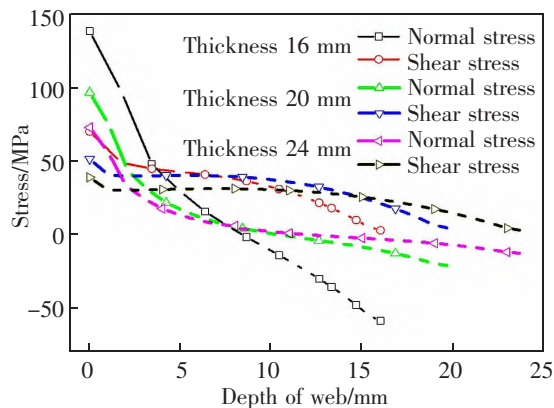
图16 不同腹板厚度下的正应力与剪应力 Fig.16 Ratio of normal stress and shear stress with different web gap thickness
