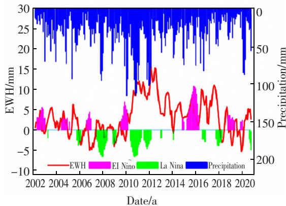
图2 墨累-达令流域等效水高与气候因素的对比 Fig.2 Comparison of EWH and climatic factors in the Murray-Darling basin
