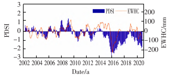
(b) Comparison of PDSI and EWHC
