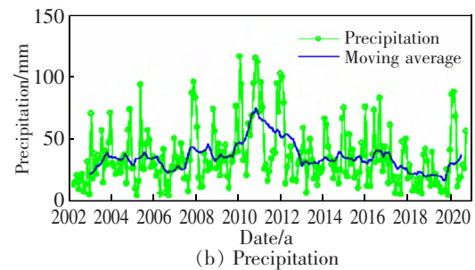
图3 墨累-达令流域等效水高和降水距平值的对比 Fig.3 Comparison of EWH and precipitation anomaly in the Murray-Darling basin
