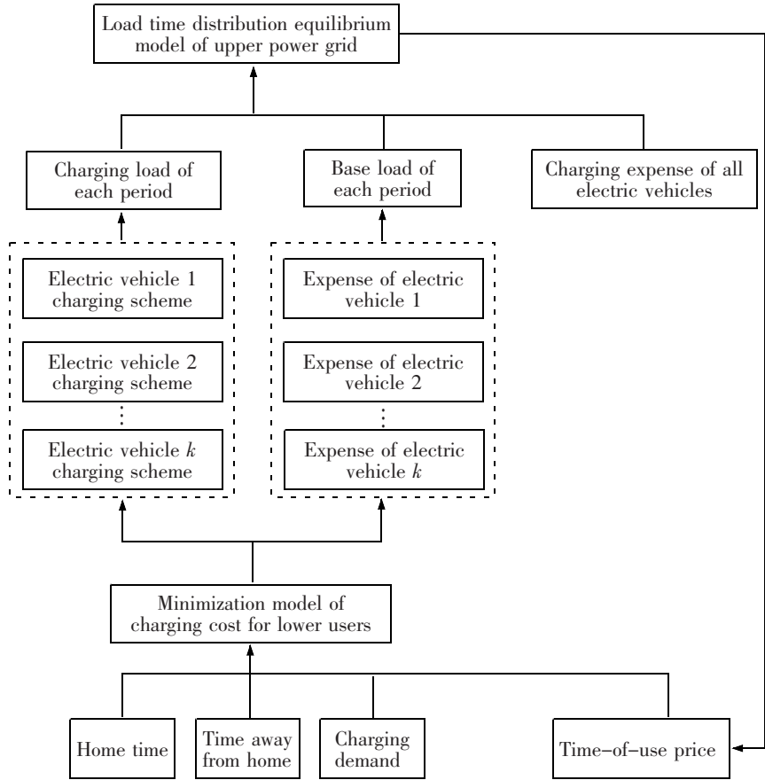
图 1 双层规划模型流程图 Fig.1 Flow chart of two-level programming model
