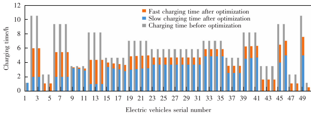
图 12 优化前后充电时长对比图 Fig.12 Comparison diagram of charging time before and after optimization
