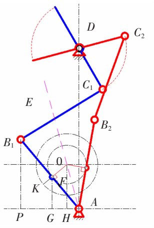
图 6 摆杆机构设计 Fig.6 Design of oscillating mechanism
