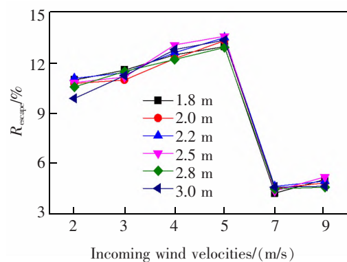
图 7 不同围挡高度和来流风速下的扬尘逃逸比 Fig.7 Dust fugitive ratios under different fence heights and incoming wind velocities
