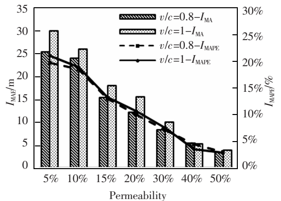
图13 不同饱和度及渗透率下最大排队长度的估计误差 Fig.13 Estimation error of the maximum queue length with different saturations and permeability
