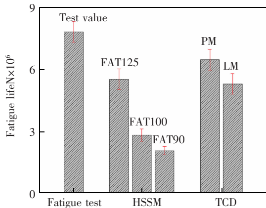
图 18 不同方法确定的疲劳寿命对比 Fig.18 Comparison of fatigue life obtained by different methods
