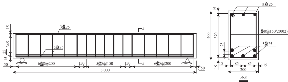
图1 RC梁的几何尺寸及配筋示意图(单位:mm) Fig. 1 Geometric size and reinforcement diagram of the RC beam(Unit: mm)
