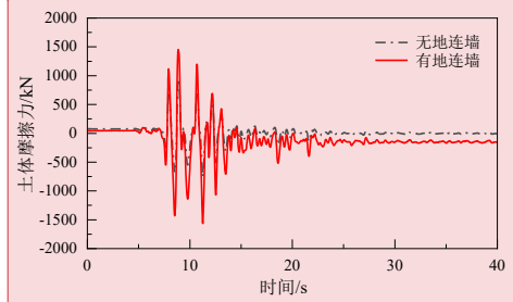
图 2 土体摩擦历时曲线 Fig.2 Time-history curves of soil friction
