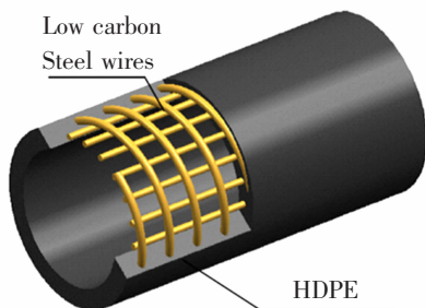
图 1 SRPE 管结构 Fig.1 The structure of SRPE tubes
