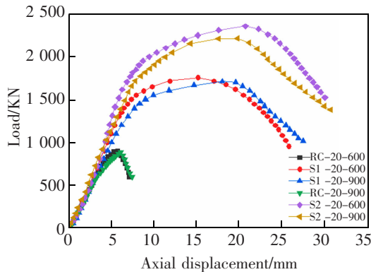
(b) Small eccentricity specimen
