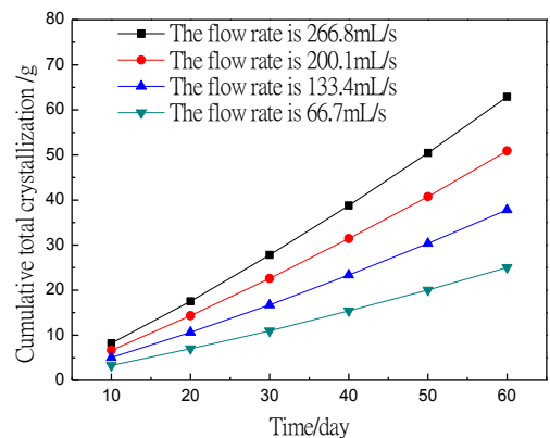
(b) I, III, V, VII. working conditions longitudinal drainage pipe crystal accumulation data per linear
