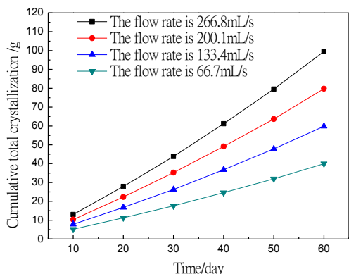
(c) I. III. V. VII. working conditions horizontal drainage pipe per linear meter crystallization accumulation data
