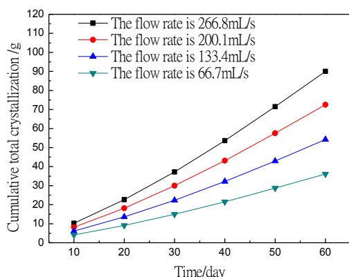
(d) I. III. V. VII. working condition joints per linear meter crystallization accumulation data
