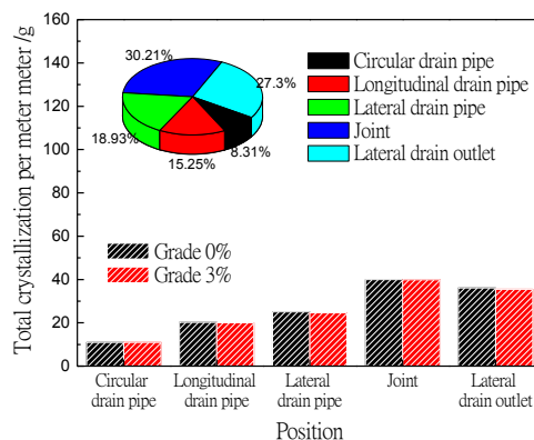
(c) Data sheet on crystallization per linear meter for each part of the tunnel when the water flow rate is 133.4mL/s
