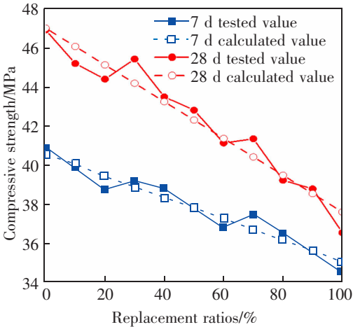
图 5 再生陶瓷粗骨料混凝土的抗压强度 Fig.5 Compressive strength of recycled ceramic coarse aggregate concrete
