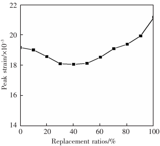
图 6 再生陶瓷粗骨料混凝土 28 d 的峰值应变 Fig.6 28 d peak strain of recycled ceramic coarse aggregate concrete
