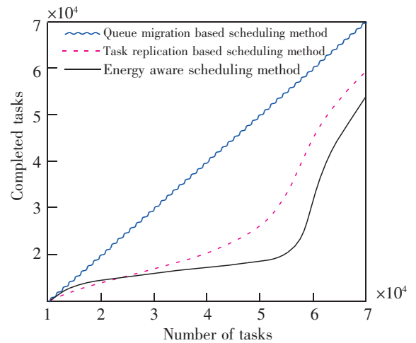
图4 3种方法任务调度完成数量对比分析 Fig.4 Comparative analysis of the task numbers scheduled by three methods
