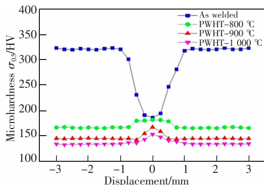
(a) Broken line diagram of microhardness
