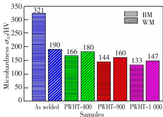
(b) Samples Histogram of microhardness
