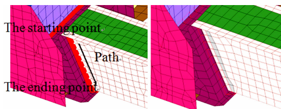
(a) Nodal path of 1# weld
