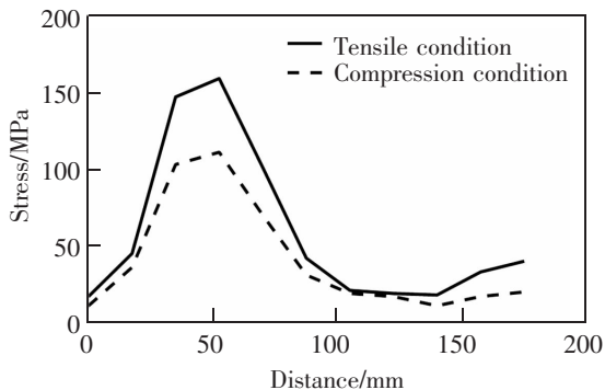
(b) The maximum equivalent structural stress value of the node on the path
