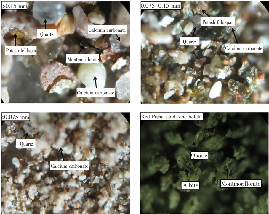
图 7 红色砒砂岩光学显微图片 (100 倍) Fig.7 Optical micrograph of different granularity red Pisha sandstone
