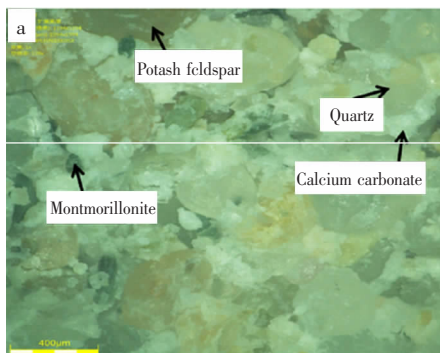
(a) White Pisha sandstone block
